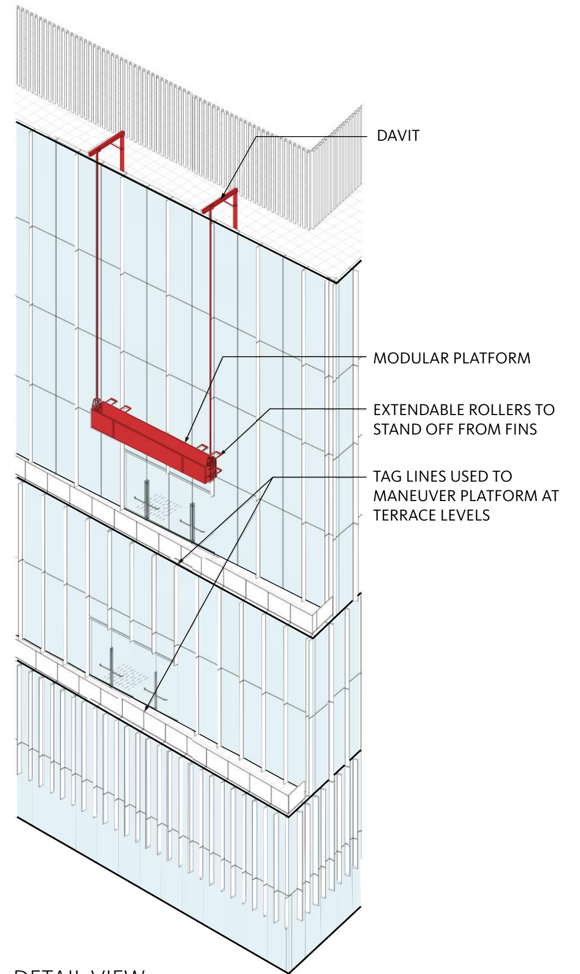
DETAIL VIEW
